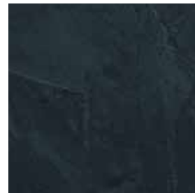
Black Grey
