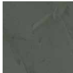
Traffic Grey
